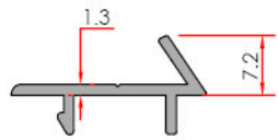
Corner Cleat İlave Kulak
