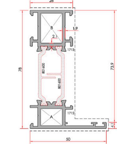
Narrow Frame Dar Kasa
