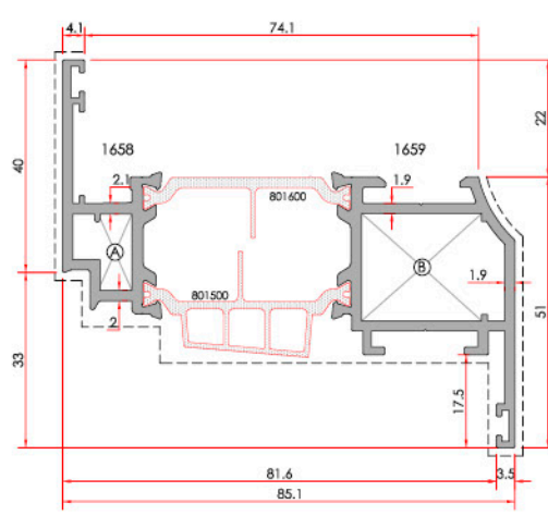
Narrow Window Sash Pencere Dar Kanat
