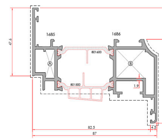
Narrow Window Sash Pencere Dar Kanat
