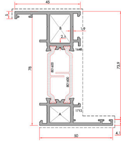
Narrow Frame Dar Kasa
