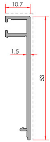
Base Cover Profile Baza Kapak Profili
