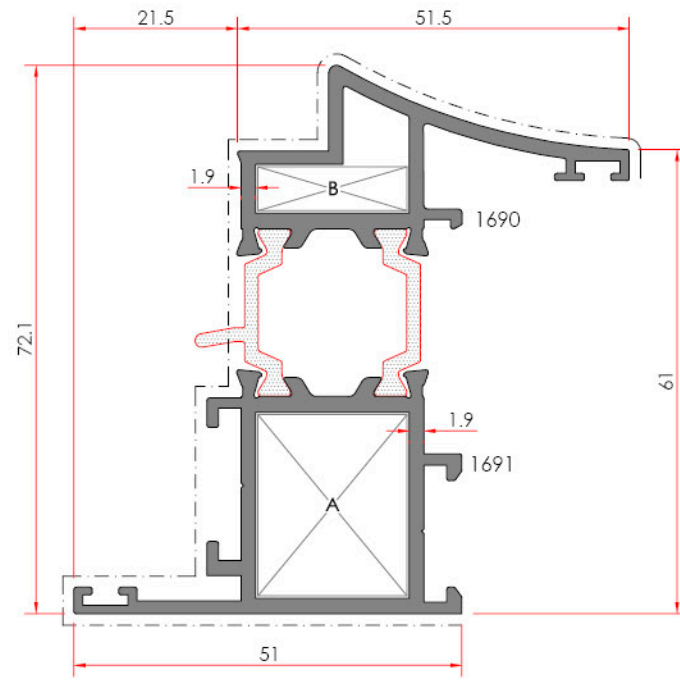
Window Sash Pencere Kanat
