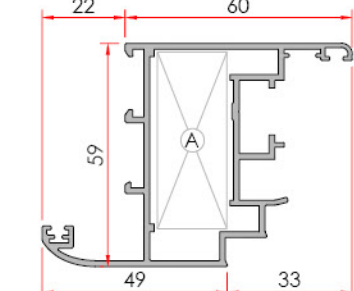
Narrow Vent Dar Kanat
