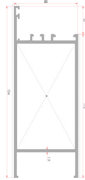
Sill Profile Etek Profili
