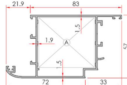
Narrow Vent Dar Kanat
