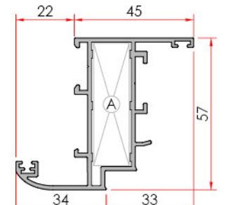
Narrow Vent Dar Kanat
