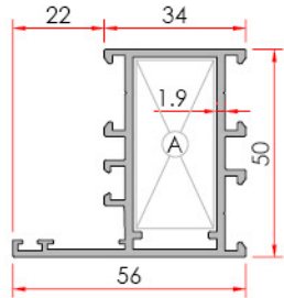
Wide Vent Geniş Kasa
