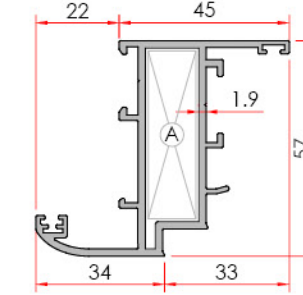
Narrow Vent Dar Kanat
