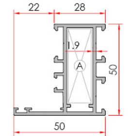
Narrow Vent Dar Kasa
