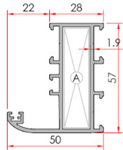
Narrow Vent Dar Kasa
