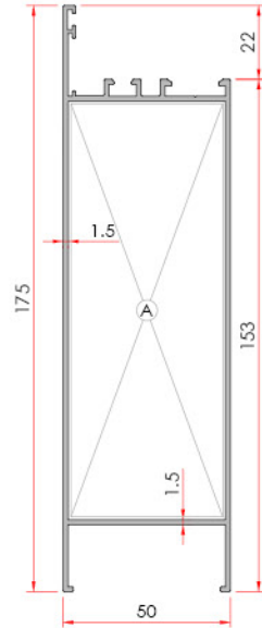
Wide Sill Profile Geniş Etek Profili
