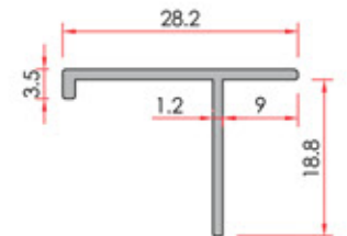
Sill Profile - T Pervaz T Profili
