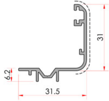
Sill Profile Pervaz Profili
