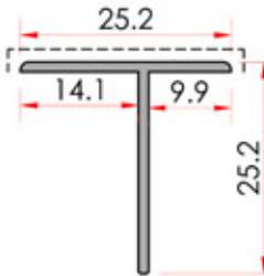
Sill Profile - T Pervaz T Profili
