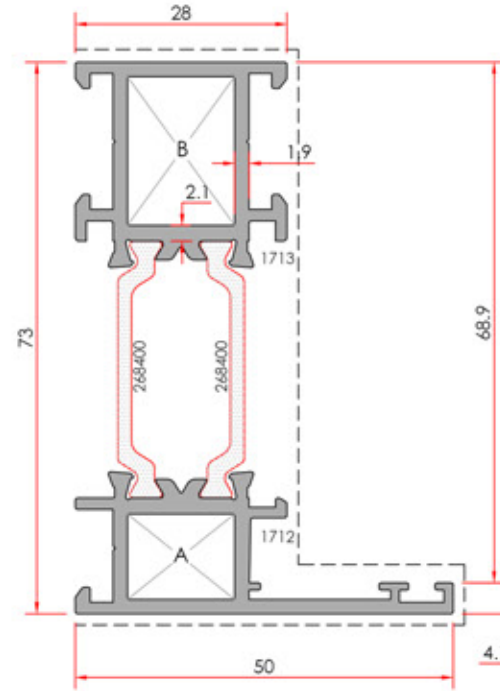
Narrow Frame Dar Kasa
