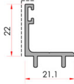
Corner Cleat İlave Kulak
