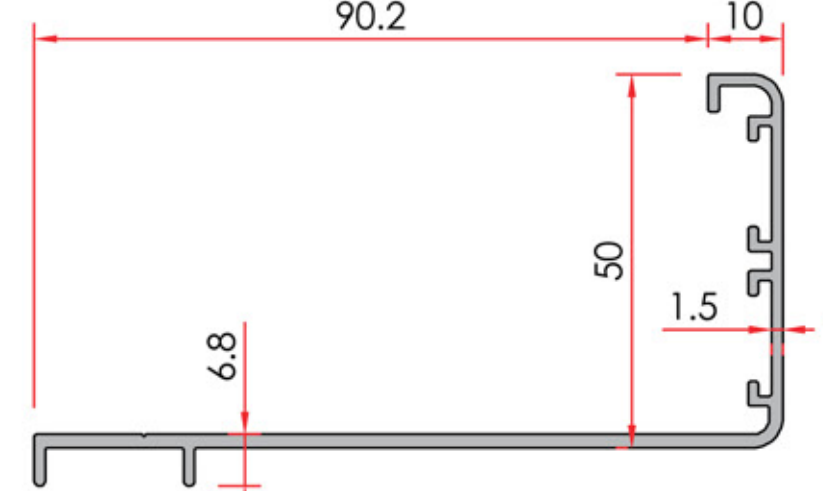
Sill Profile Pervaz Profili
