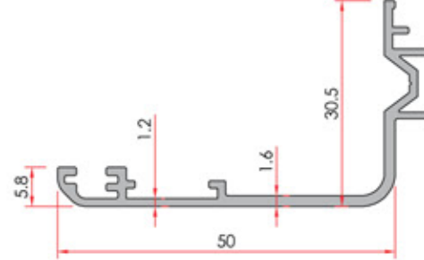
Sill Profile Pervaz Profili
