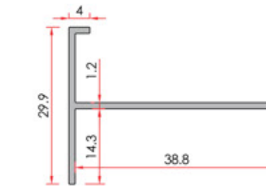
Sill Profile - T Pervaz T Profili
