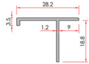
Sill Profile - T Pervaz T Profili
