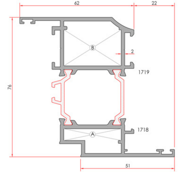
Vent Profile Kanat Profili
