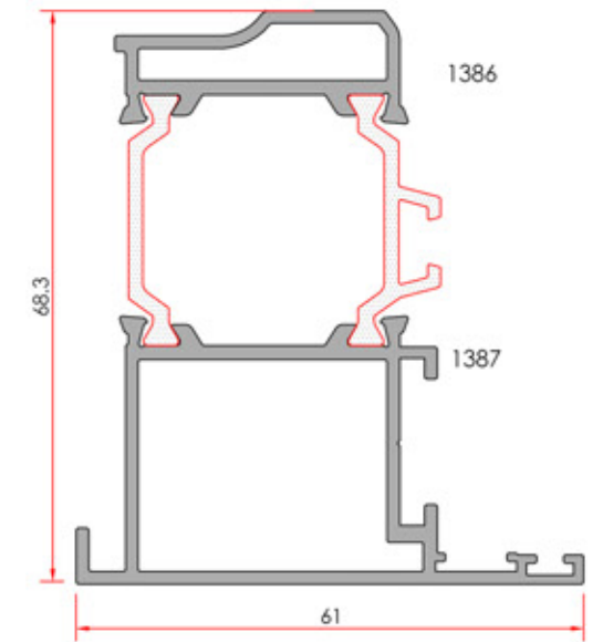
Pivoted Adapter Pivot Adaptörü
