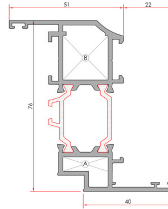
Narrow Vent Dar Kanat
