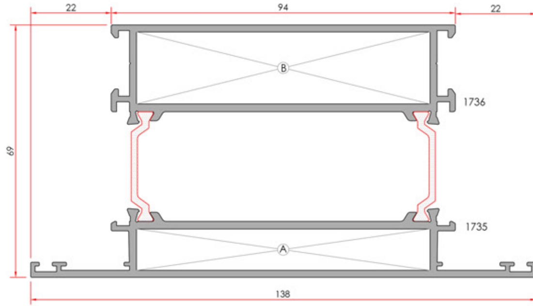
Meeting Base Profile Orta Baza Profili
