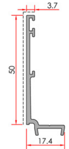
Sill Profile Pervaz Profili
