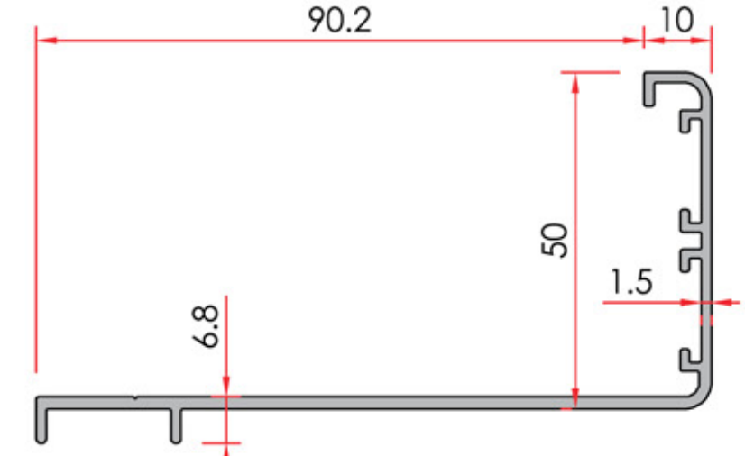
Sill Profile Pervaz Profili
