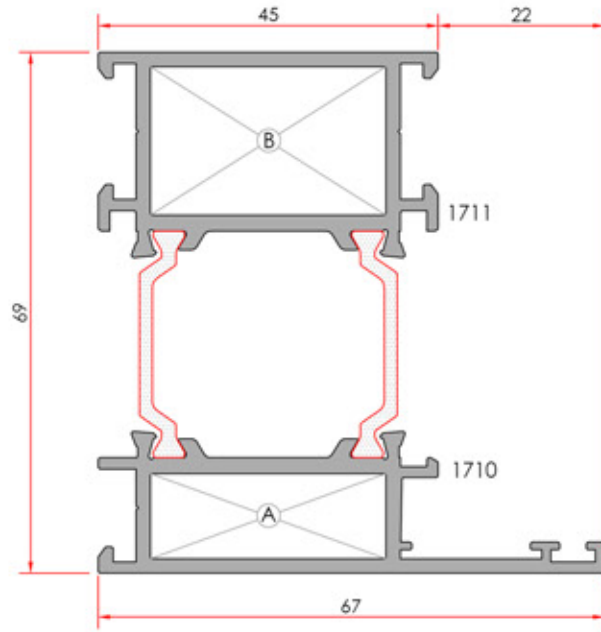
Frame Profile Kasa Profili
