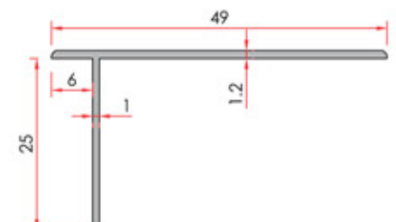
Sill Profile - T Pervaz T Profili
