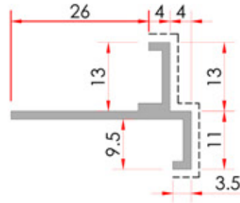
Sill Profile Pervaz Profili
