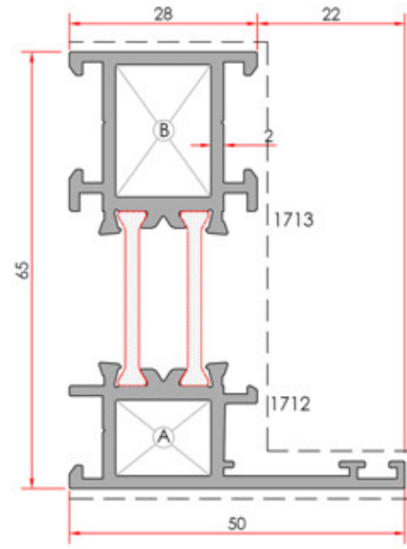
Narrow Frame Dar Kasa
