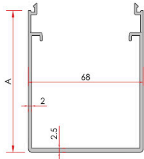
Bottom Cover Profile Alt Kapak Profili
