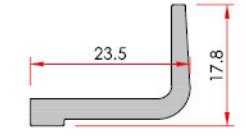
Glazing Cleat Cam Takozu
