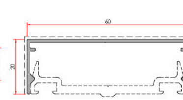
Cover Dikey Kapak
