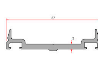
Cover Basla Kapak
