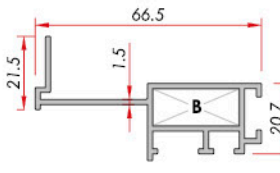
Spandrel Panel Spandrel Paneli
