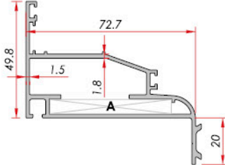
Hidden Wing Frame Gizli Kanat Kasa Panel
