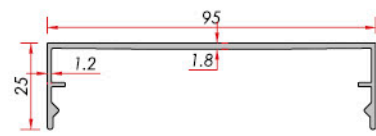
Cover Dikey Kapak
