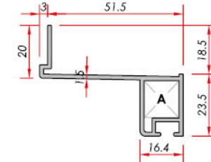
Single Glass Panel Tek Cam Paneli
