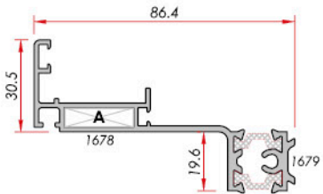
Hidden Wing Frame Gizli Kanat Kasa Panel
