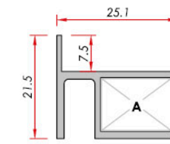
Single Glass Panel Tek Cam Paneli
